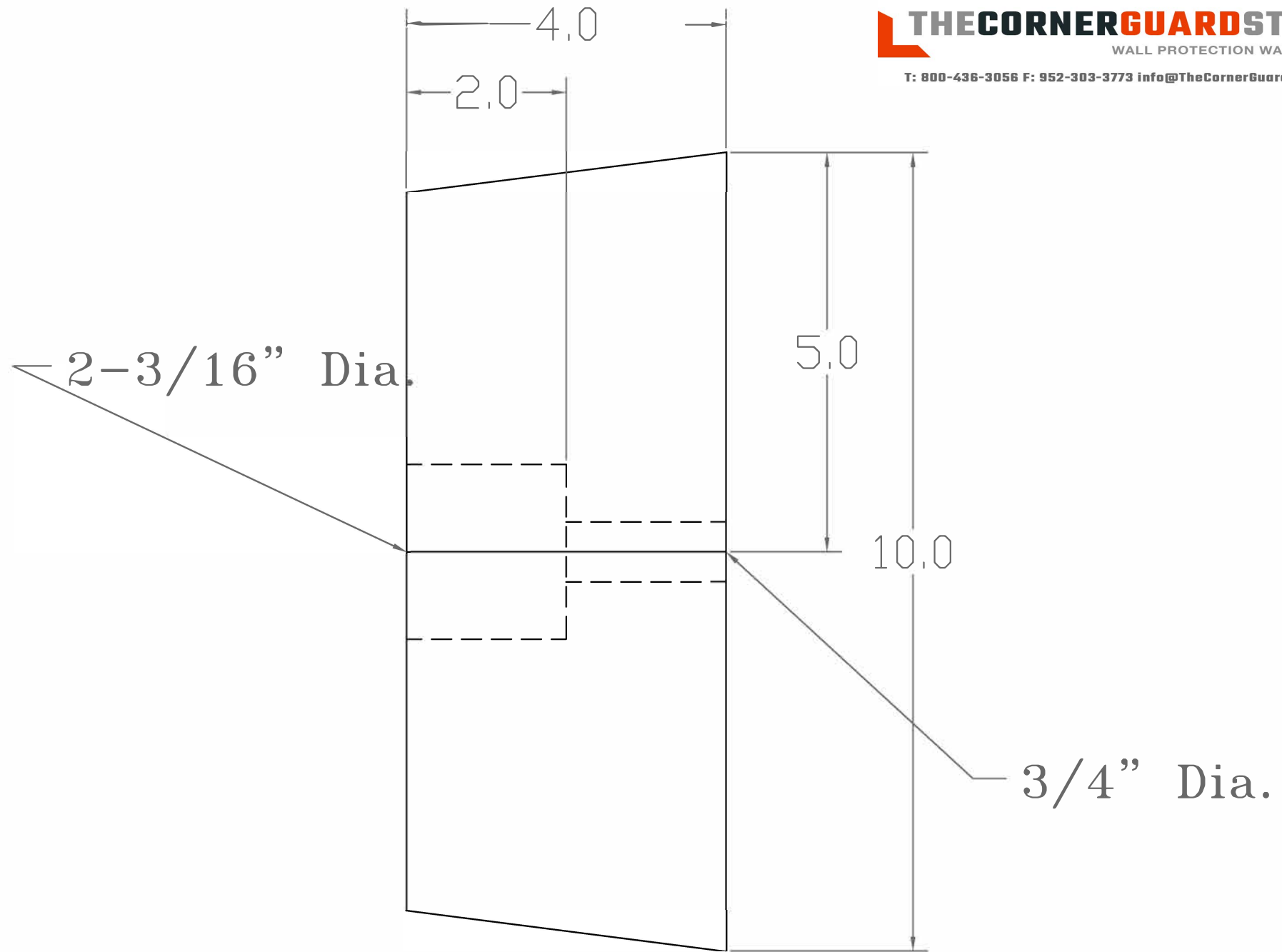
DB-13 Molded Bumper Side View
